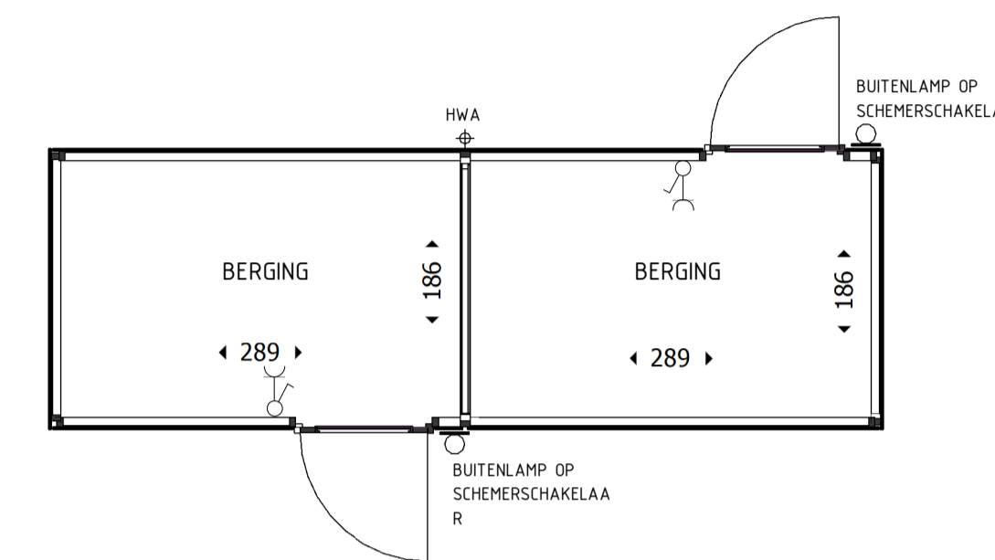
PLATTEGROND 150 BERGINGTYPE C1' / C2' / C3' / C8
